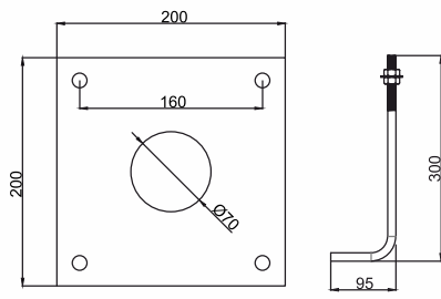
FOUNDATION TEMPLATE M12 J-BOLT
