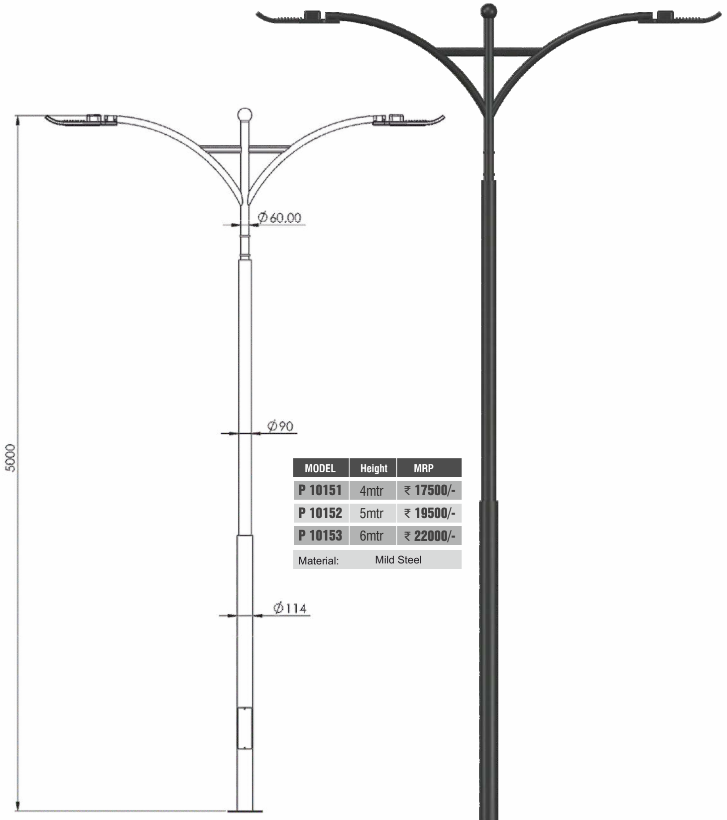
Double Arm Pole
