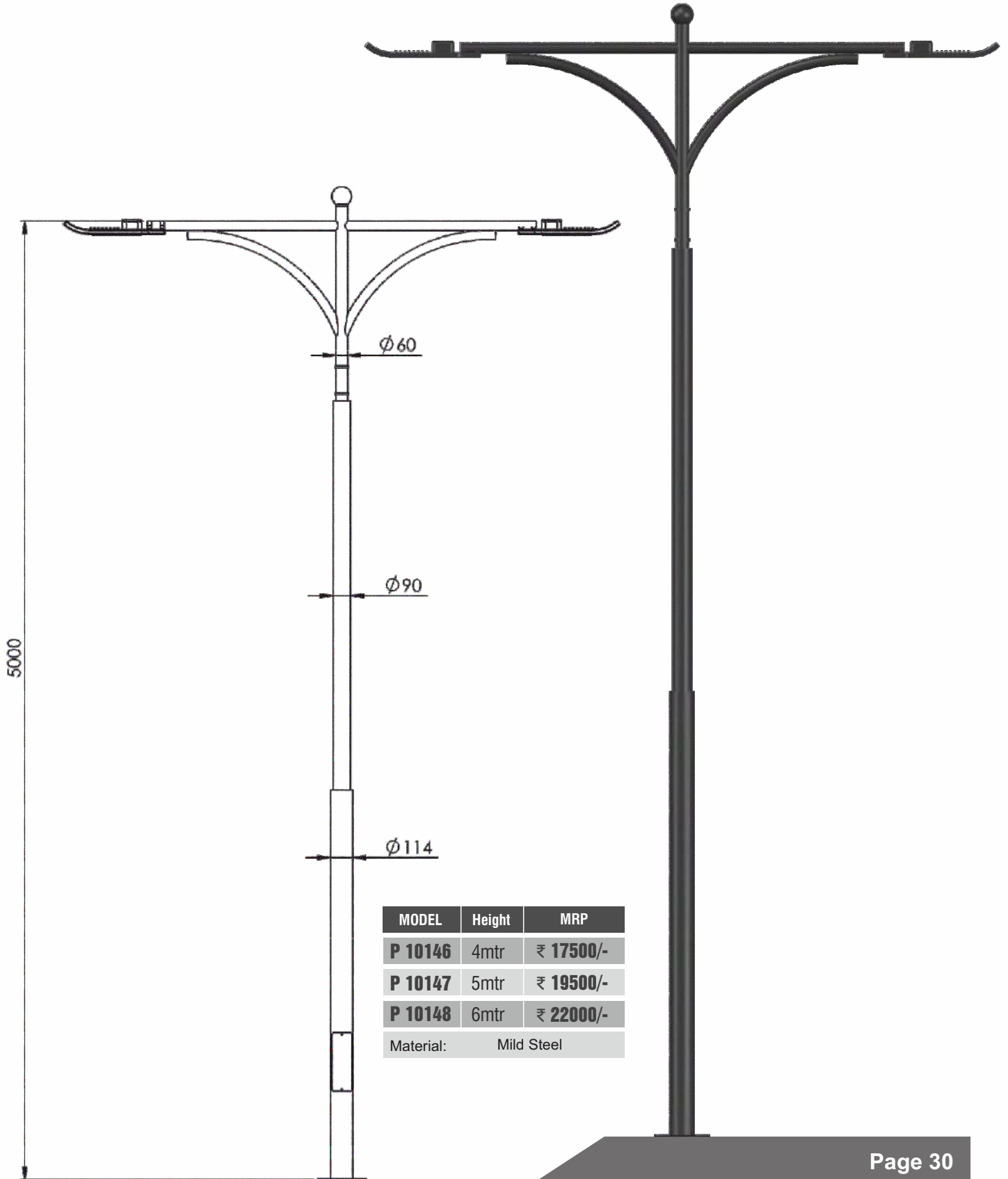
Double Arm Pole
